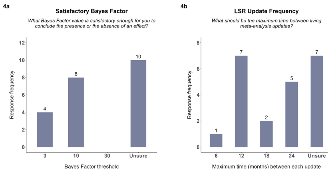
Fig. 4. Questionnaire items from the first questionnaire with multiple response options. Questions are shown under each subtitle ( n = 22 ). LSR = Living systematic review. Bayes Factor = statistical measure comparing how well competing hypothesis explains the data. Bayes Factor can quantify evidence for both presence and absence of an effect.
