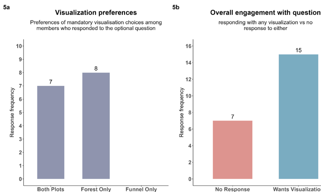
Fig. 5. Meta-analysis Visualization Preferences. Questionnaire items from the first questionnaire with multiple response options. ( n = 22 ). The responders of the first questionnaire had the optional question “Which of these meta-analysis visualisations should be mandatory? (Select any that you think should be mandatory)”. The response options were Forest plot and Funnel plot.
